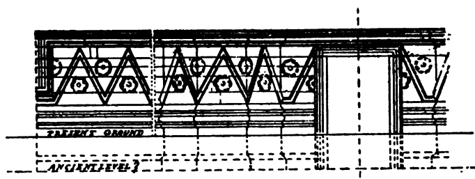
FIG. 32. Diagram of lower storey of the Palace at Mashita in Moab. The whole is elaborately carved with foliage, birds, and beasts.
